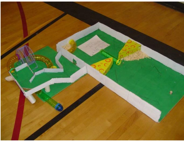
Asteroid Belt
