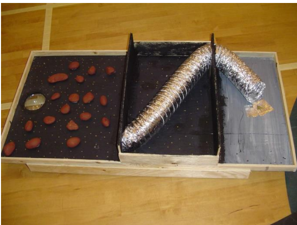
Asteroid Belt
